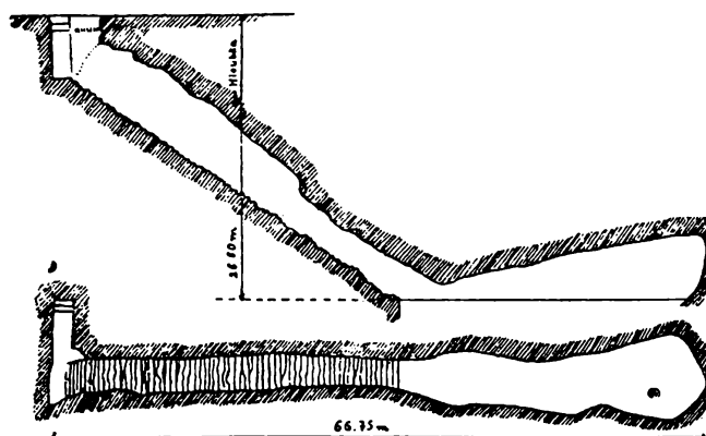
Obr. 272. Tunel v Gezer.
