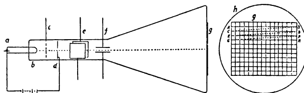
Obr. 3. Katodová trubice.
